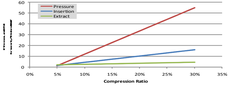
Dimensional Compression Ratio - Seal Performance
