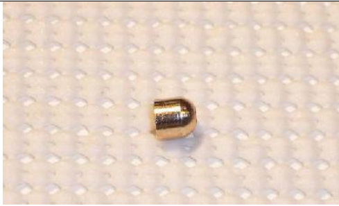
Part number: 30245-1 (X1344-) Button-Radius End; ¼ Dia. x .25 long: Plated Steel Compatible with: .054, .062, .075 core
